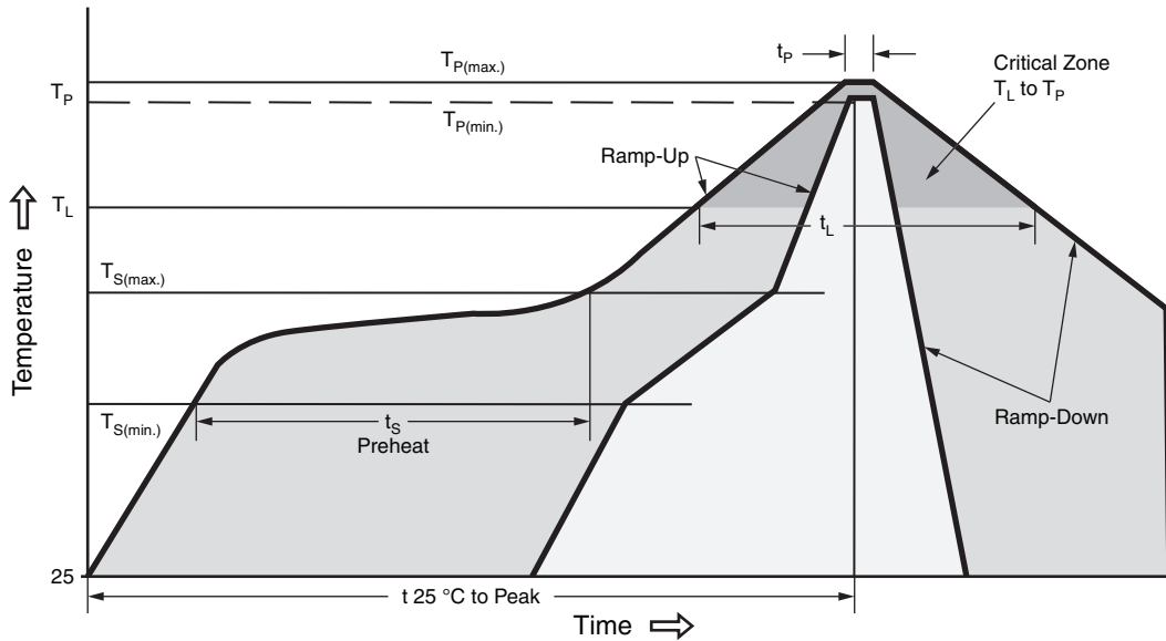
Classification Reflow Profile
