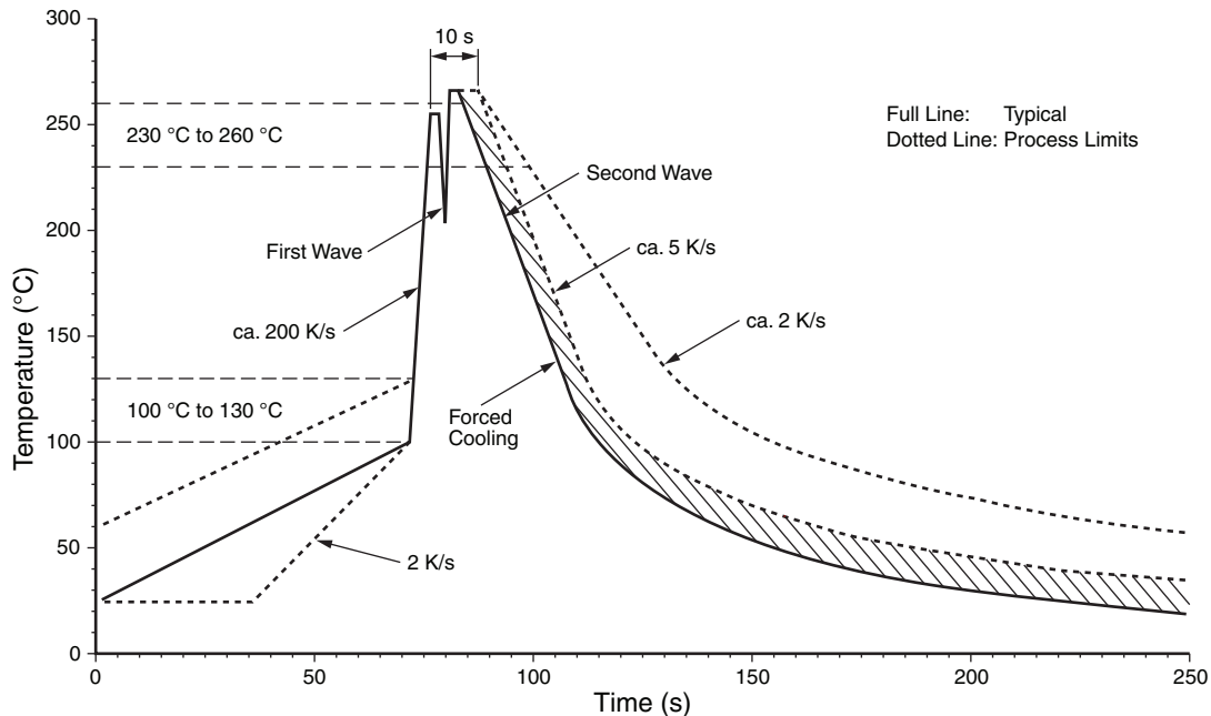
Double-Wave-Soldering, Temperature/Time - Profile (Lead-Temperature)
